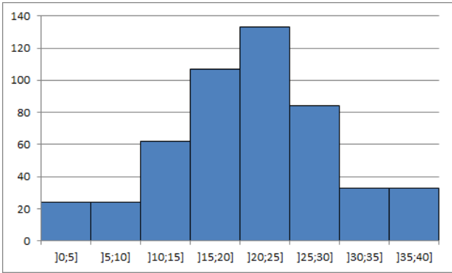
FIGURE 10.13 – Histogramme correct.
